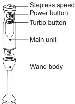
Wand Attachment
